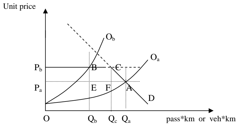
Figure 1 – Behaviour of the PC users on the Maréchaux ' boulevards (before and after the project)
