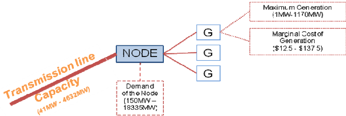
Figure 2 – Detailed scheme of Transmission Network
