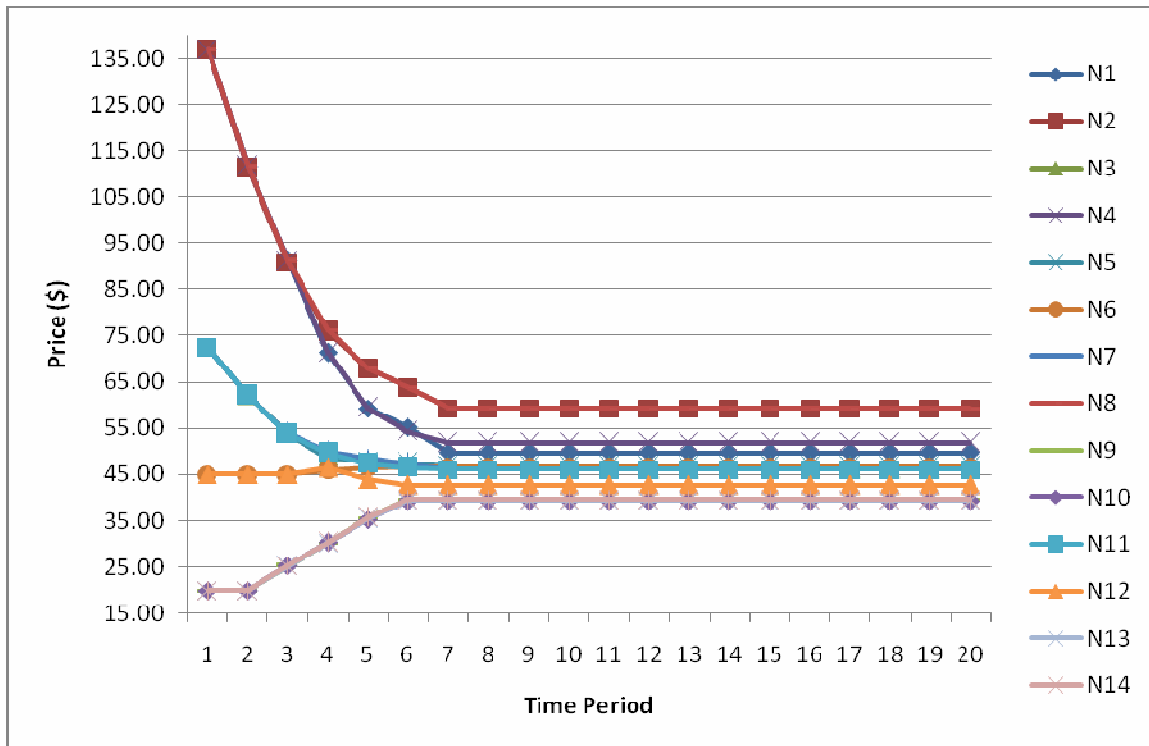
Figure 6 – Price development for PJM Classic region
